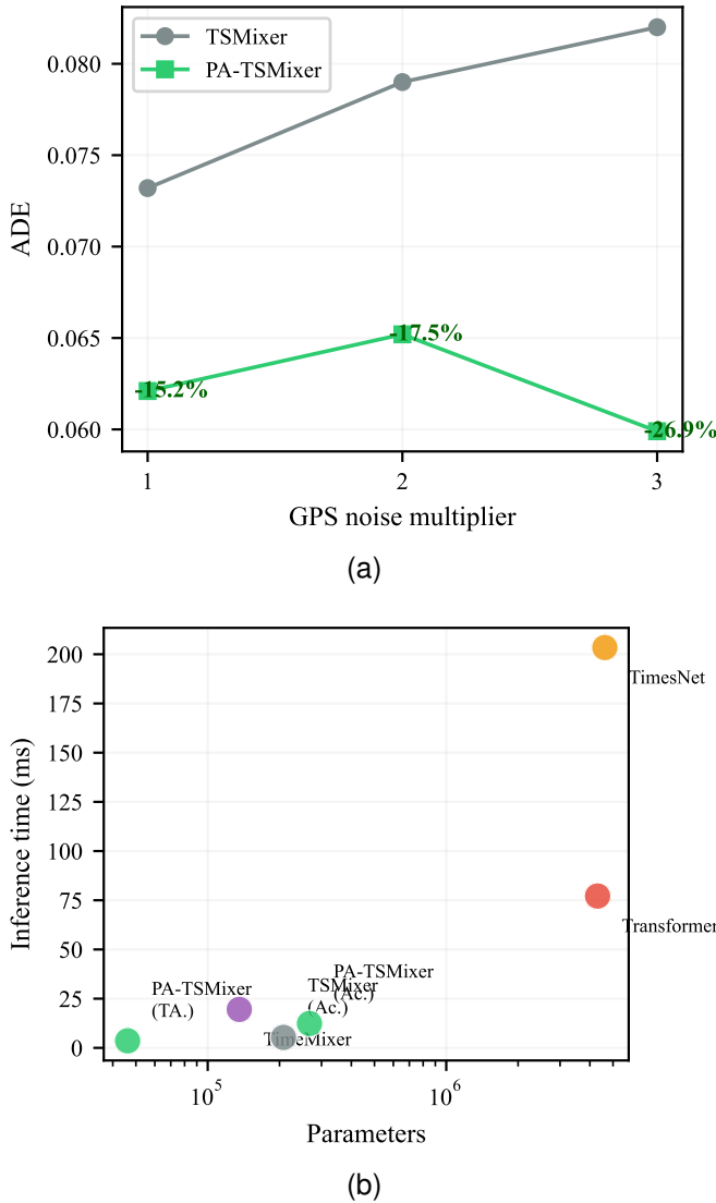
Fig. 5. (a) Noise robustness: PA-TSMixer’s relative advantage grows from -15.2\% to -26.9\% as GPS noise triples. (b) Computational efficiency: PA-TSMixer occupies the favorable lower-left region.
