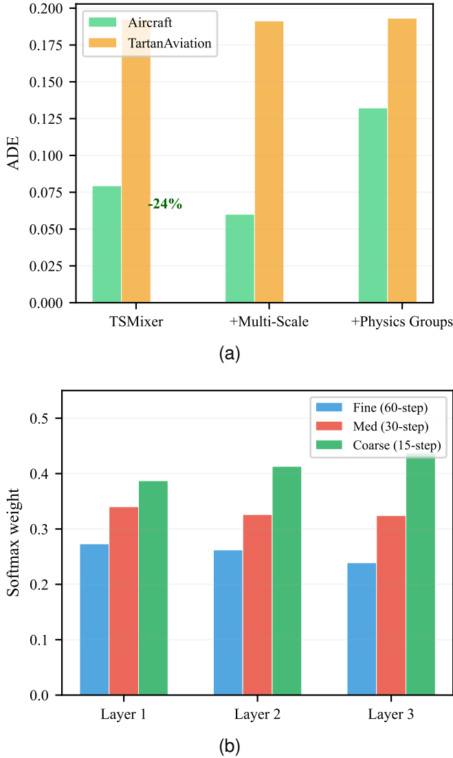
Fig. 4. (a) Component ablation with consistent model capacity. Multi-scale temporal mixing provides a 24% ADE reduction on Aircraft. (b) Learned branch weights after softmax normalization, showing progressive shift toward coarser scales in deeper layers.
