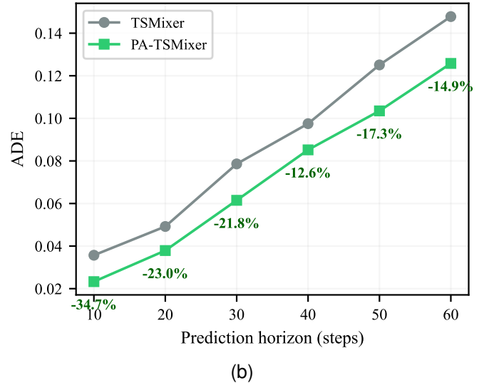
Fig. 2. (a) Per-maneuver-type ADE comparison. PA-TSMixer achieves the largest relative improvement on CTRV trajectories ( -36.9\% ). (b) ADE across prediction horizons. PA-TSMixer consistently outperforms TSMixer.
