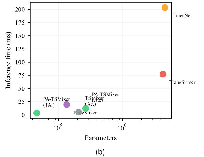
Fig. 6. (a) Noise robustness: PA-TSMixer's relative advantage grows from -15.2\% to -26.9\% as GPS noise triples. (b) Computational efficiency: PA-TSMixer occupies the favorable lower-left region.
