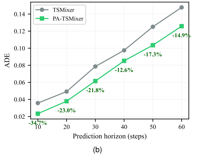
Fig. 3. (a) Per-maneuver-type ADE comparison. PA-TSMixer achieves the largest relative improvement on CTRV trajectories ( -36.9\% ). (b) ADE across prediction horizons. PA-TSMixer consistently outperforms TSMixer.
