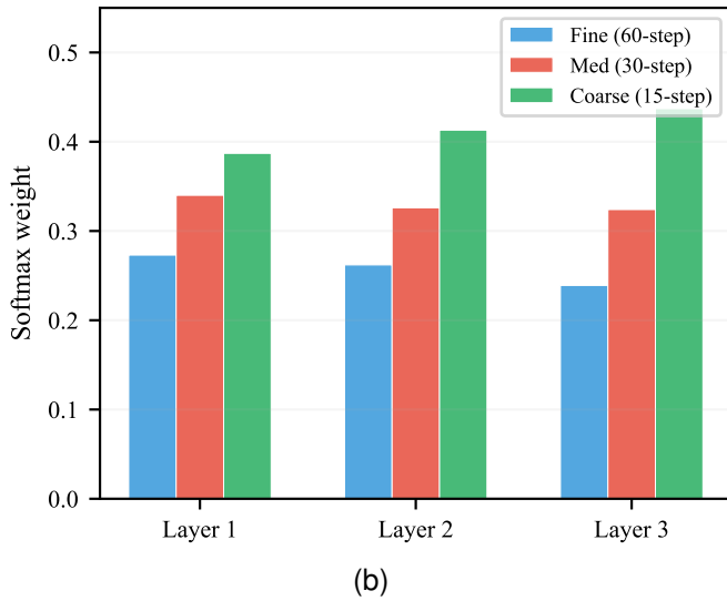
Fig. 5. (a) Component ablation with consistent model capacity. Multi-scale temporal mixing provides a 24% ADE reduction on Aircraft. (b) Learned branch weights after softmax normalization, showing progressive shift toward coarser scales in deeper layers.
