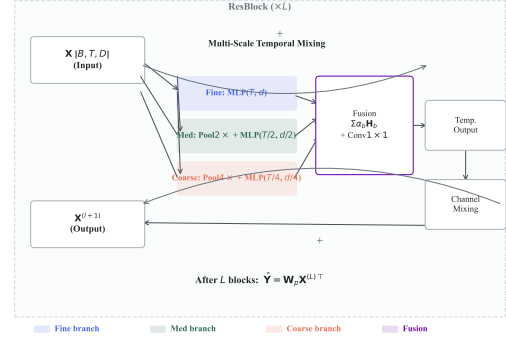
Fig. 2. PA-TSMixer architecture. Each ResBlock contains a multi-scale temporal mixing module with three parallel branches (fine, medium, coarse) operating at progressively downsampled resolutions, followed by standard channel mixing.
