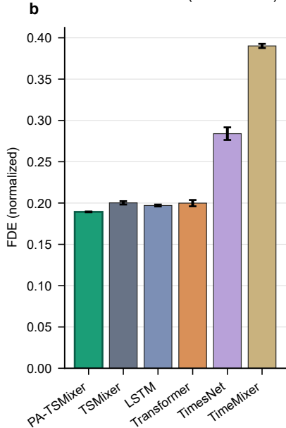
TrajAir clean-window benchmark (three seeds)
