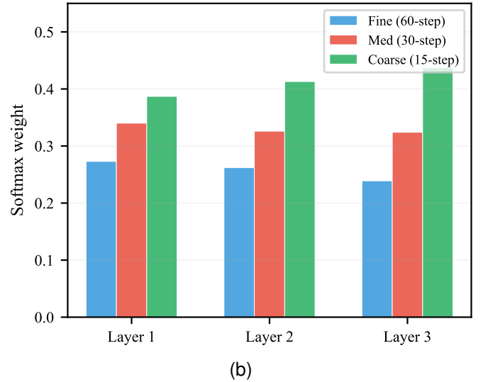
Fig. 5. (a) Component ablation with consistent model capacity. Multi-scale temporal mixing provides a 24% ADE reduction on Aircraft. (b) Learned branch weights after softmax normalization, showing progressive shift toward coarser scales in deeper layers.
