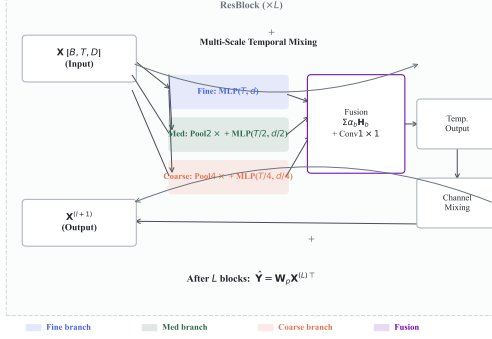
Fig. 2. PA-TSMixer architecture. Each ResBlock contains a multi-scale temporal mixing module with three parallel branches (fine, medium, coarse) operating at progressively downsampled resolutions, followed by standard channel mixing.
