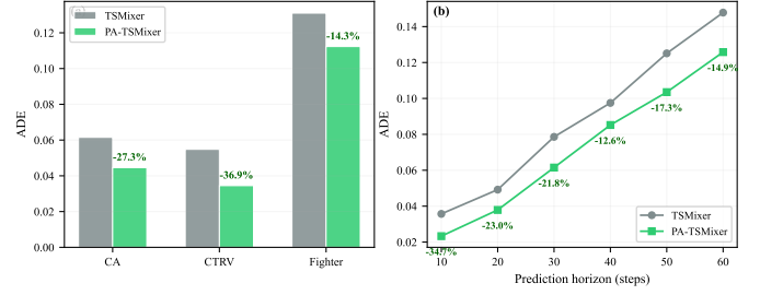
Fig. 2. (a) Per-maneuver-type ADE comparison. PA-TSMixer achieves the largest relative improvement on CTRV trajectories ( -36.9\% ). (b) ADE across prediction horizons. PA-TSMixer consistently outperforms TSMixer, with the largest advantage at short horizons ( -34.8\% at 10 steps).
