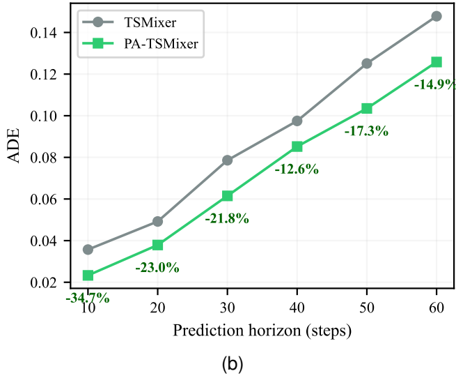
Fig. 2. (a) Per-maneuver-type ADE comparison. PA-TSMixer achieves the largest relative improvement on CTRV trajectories ( -36.9\% ). (b) ADE across prediction horizons. PA-TSMixer consistently outperforms TSMixer.
