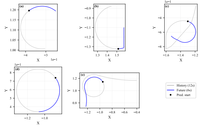
Fig. 3. Representative trajectory predictions on the Aircraft dataset. (a)–(e) Five test examples with increasing displacement magnitude. Gray: 12s history. Blue: 6s ground-truth future. Black dot: prediction start.
