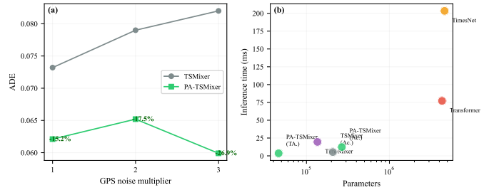
Fig. 5. (a) Noise robustness: PA-TSMixer’s relative advantage grows from −15.2% to −26.9% as GPS noise triples, due to implicit low-pass filtering in the pooled branches. (b) Computational efficiency: PA-TSMixer occupies the favorable lower-left region with low parameter count and fast inference.
