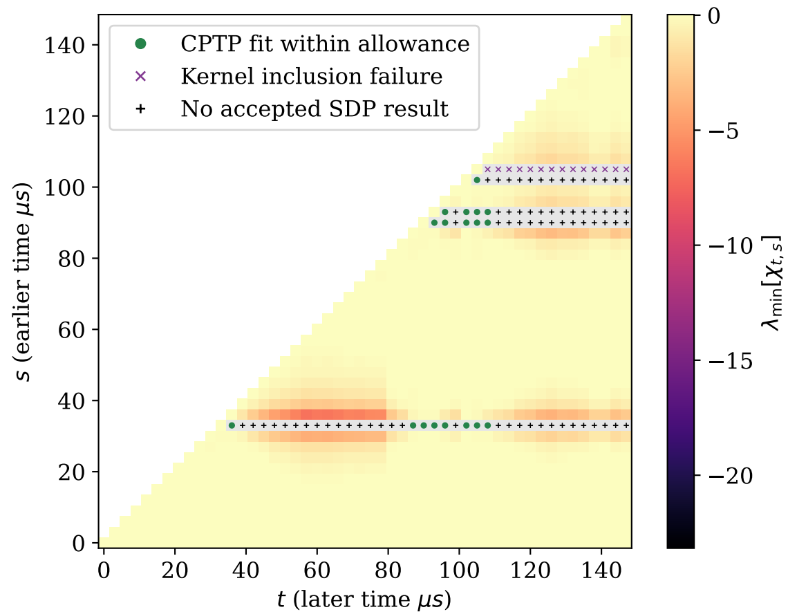
Effective-rank protocol
