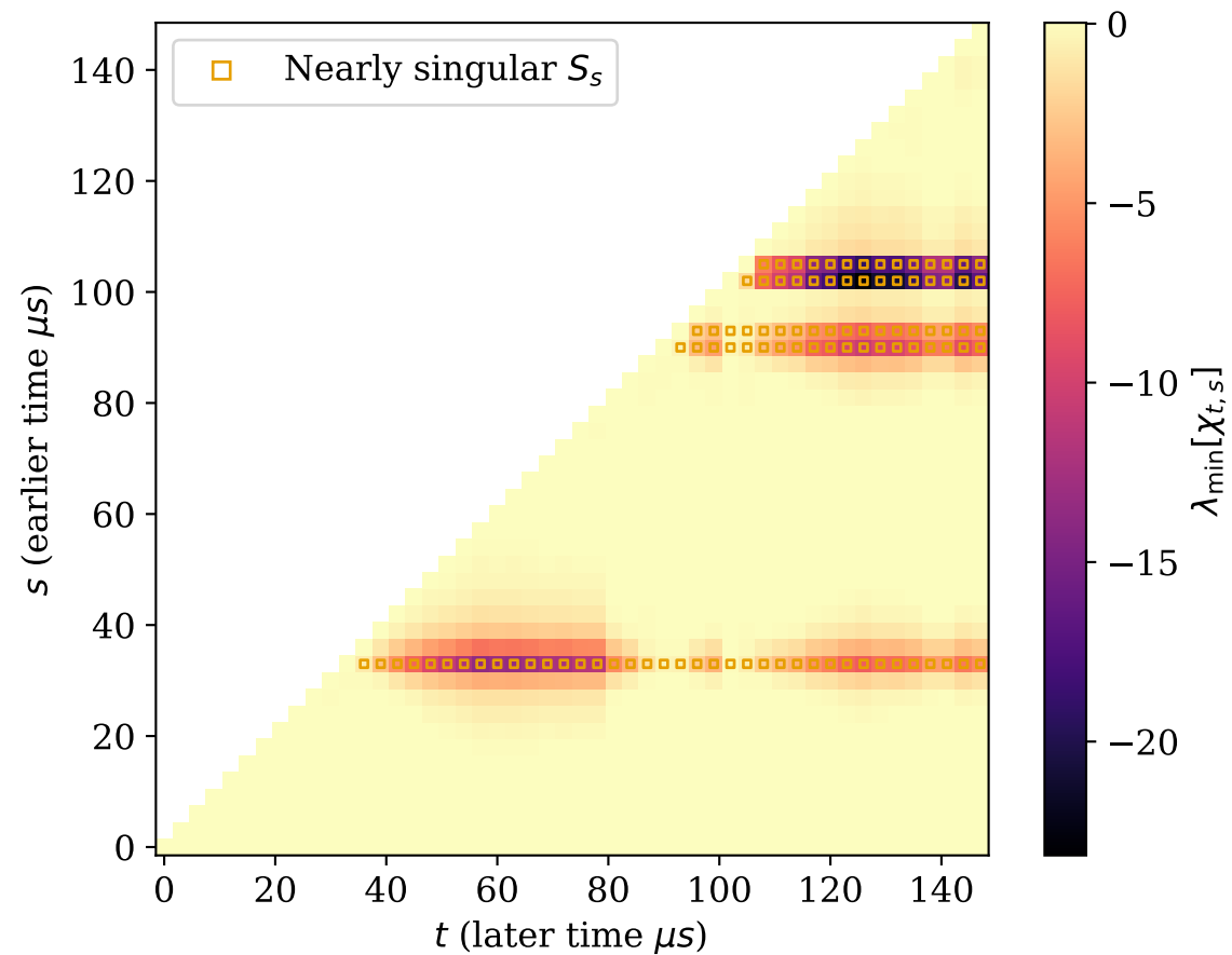
Raw inverse (before rank truncation)
