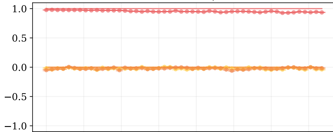
Initial state |0\rangle
