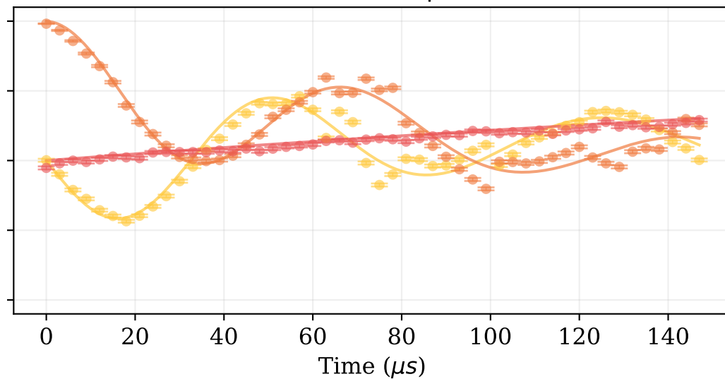
Initial state |+i\rangle
