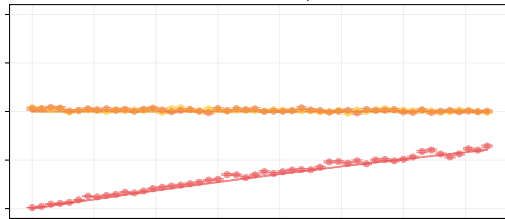
Initial state |1\rangle
