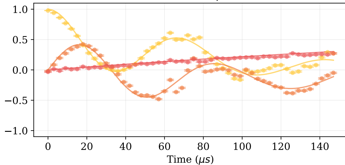
Initial state |+\rangle
