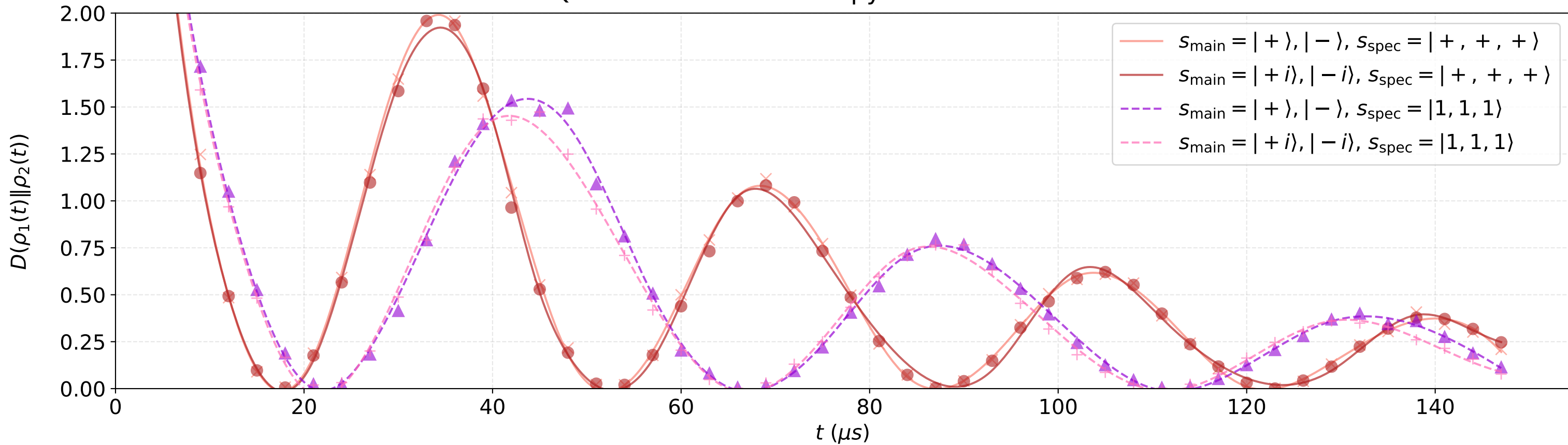
Quantum Relative Entropy between two states
