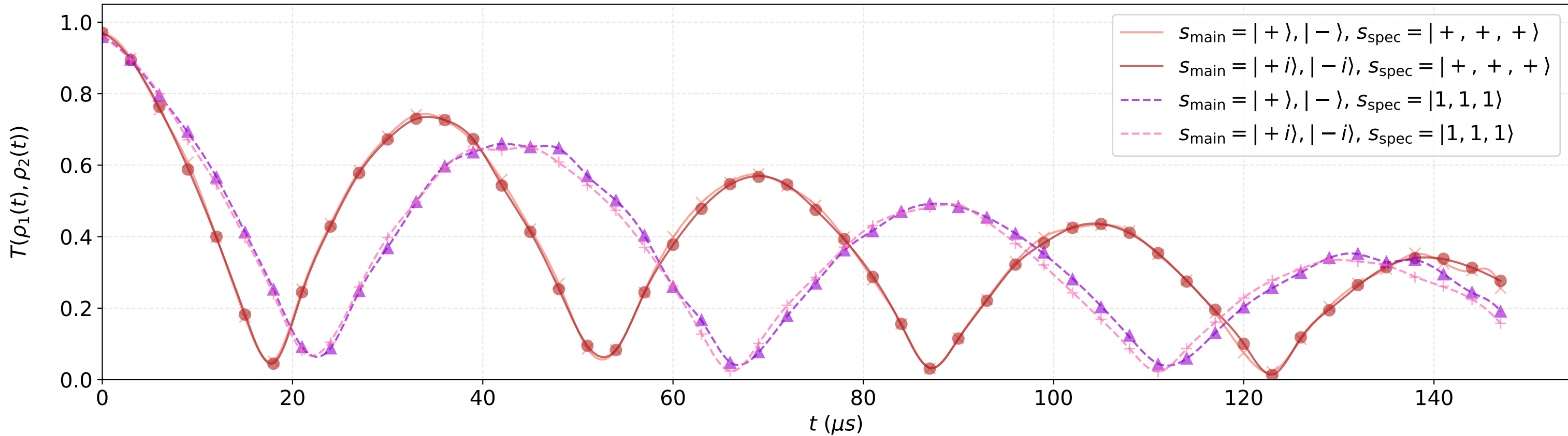
Trace Distance between two states
