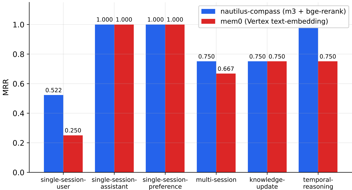
LongMemEval-S subset 12: per-question-type MRR nautilus-compass (m3+rerank) vs mem0 (Vertex), n=12, same dataset
