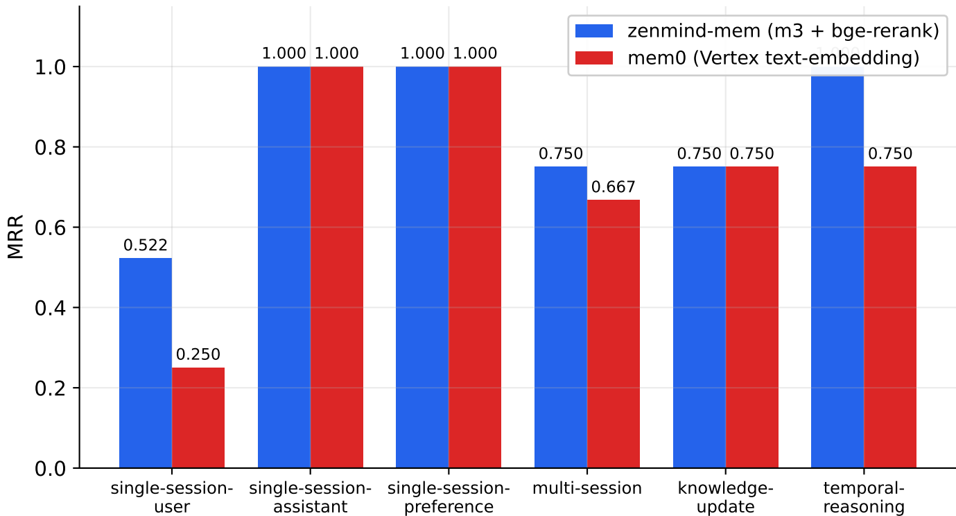
LongMemEval-S subset 12: per-question-type MRR zenmind-mem (m3+rerank) vs mem0 (Vertex), n=12, same dataset
