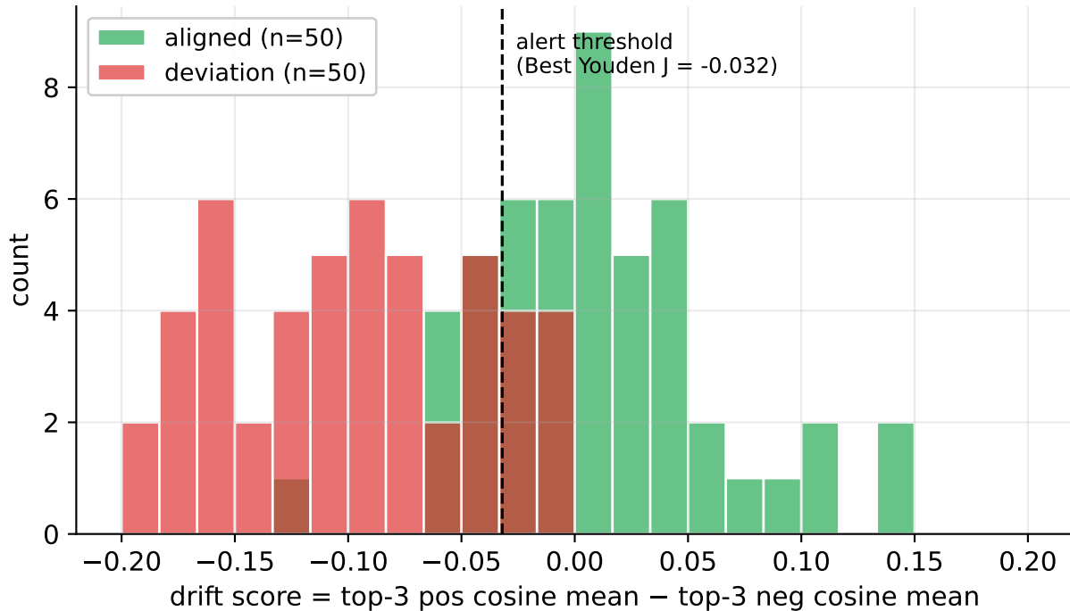
Drift score distribution: aligned vs. deviation prompts (zenmind-mem v0.7.1 · bge-m3 + 25 pos + 35 neg anchors · ROC AUC = 0.9232)
