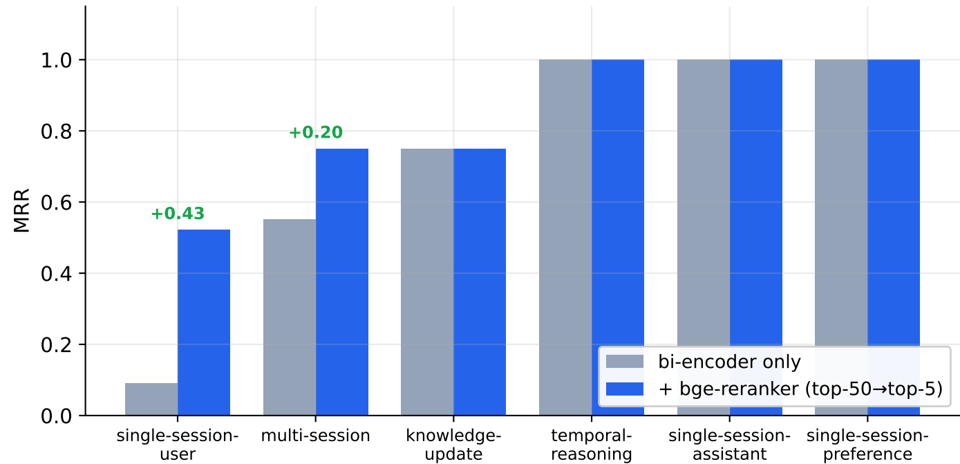
Reranker lift by question type (LongMemEval-S subset 12) 5x improvement on hardest type (single-session-user)
