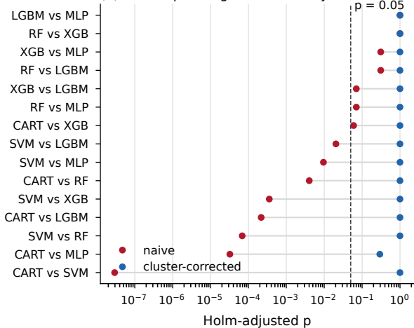
(b) 8 of 15 pairs significant naively, 0 of 15 after clustering
