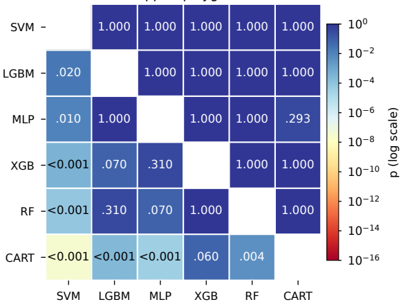
(a) Holm-adjusted McNemar p
