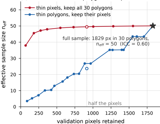
(c) information lives in polygons, not pixels
