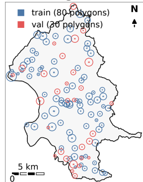
(a) training and validation polygons
