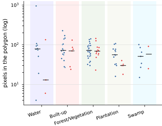
(b) cluster size: pixels per polygon
