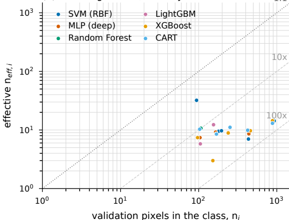
(d) the design effect, class by class
