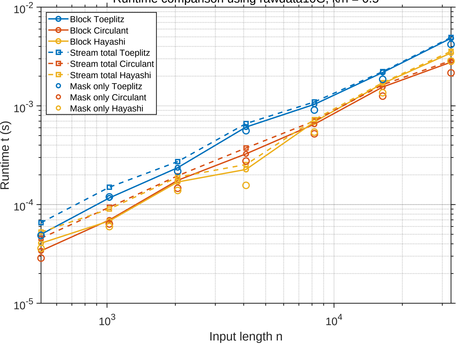
Runtime comparison using rawdata10G, k/n = 0.5
