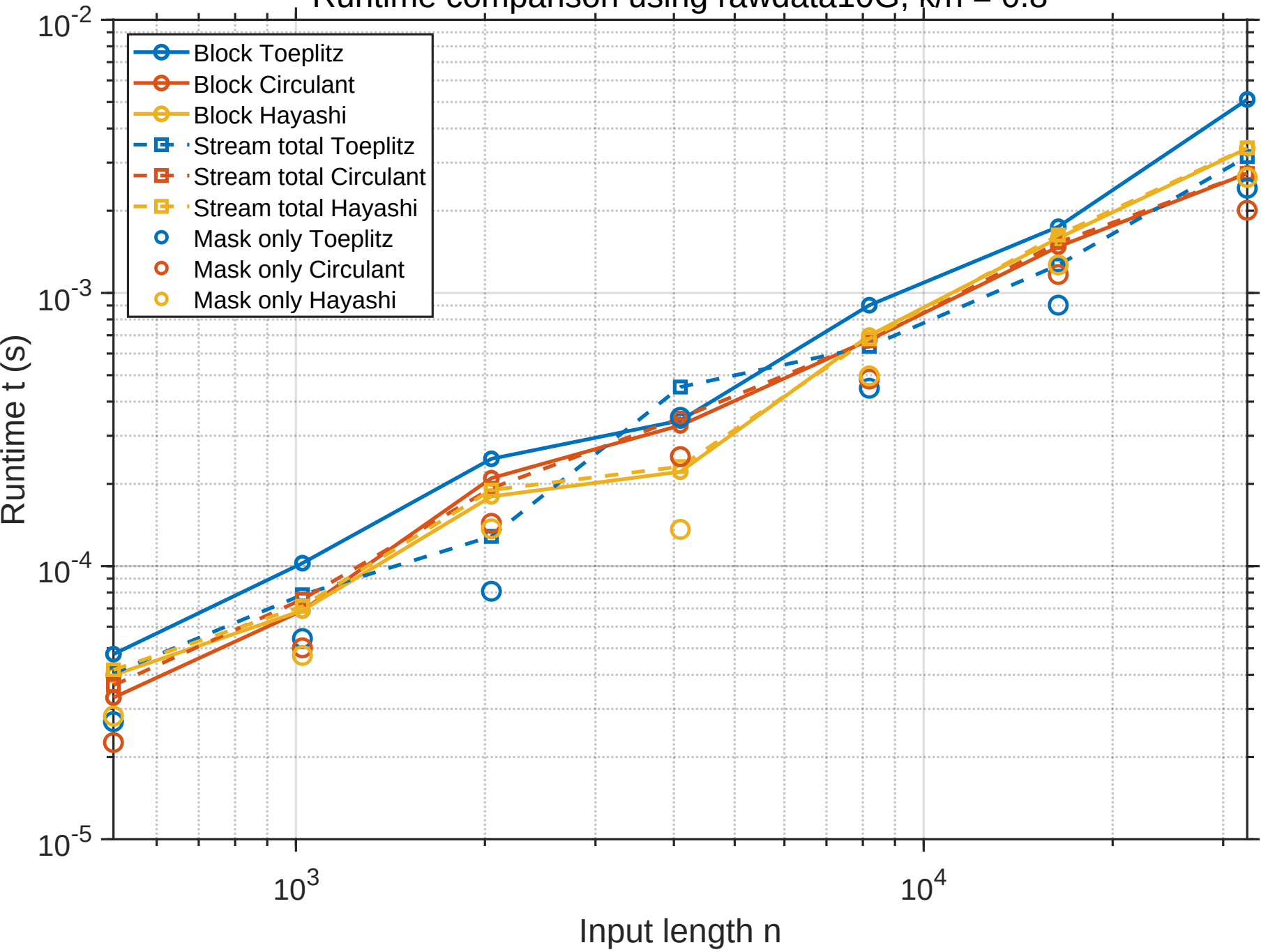
Runtime comparison using rawdata10G, k/n = 0.8
