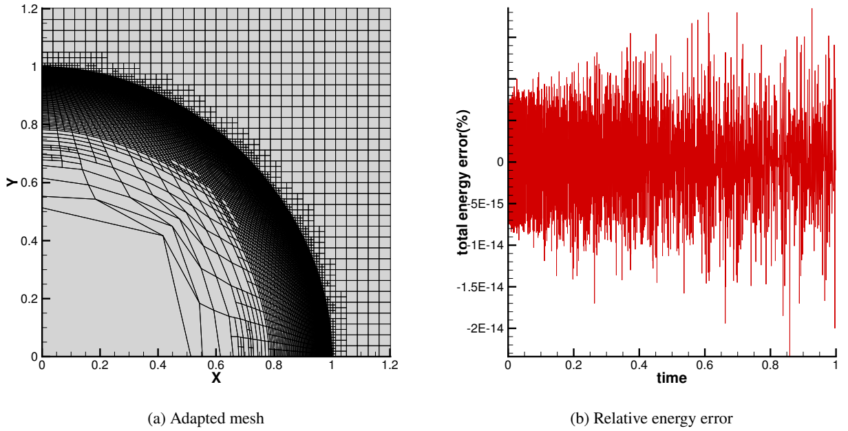
Figure 9: Sedov blast wave results under levels 5–7 mesh, and (b) time history of the total energy relative error, confirming energy conservation near machine precision.
