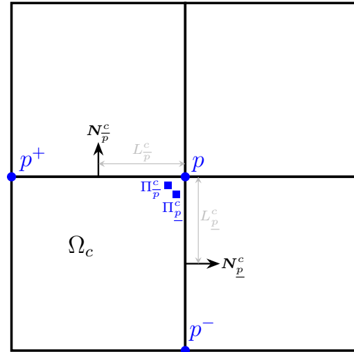
Figure 1: Schematic of the notation for a generic quadrilateral cell \Omega_c , showing the subcell parameters (L_{\underline{p}}^c, \mathbf{N}_{\underline{p}}^c, \Pi_{\underline{p}}^c) and (L_{\underline{p}}^c, \mathbf{N}_{\underline{p}}^c, \Pi_{\underline{p}}^c) associated with node p and its neighbors p^+ and p^- .
