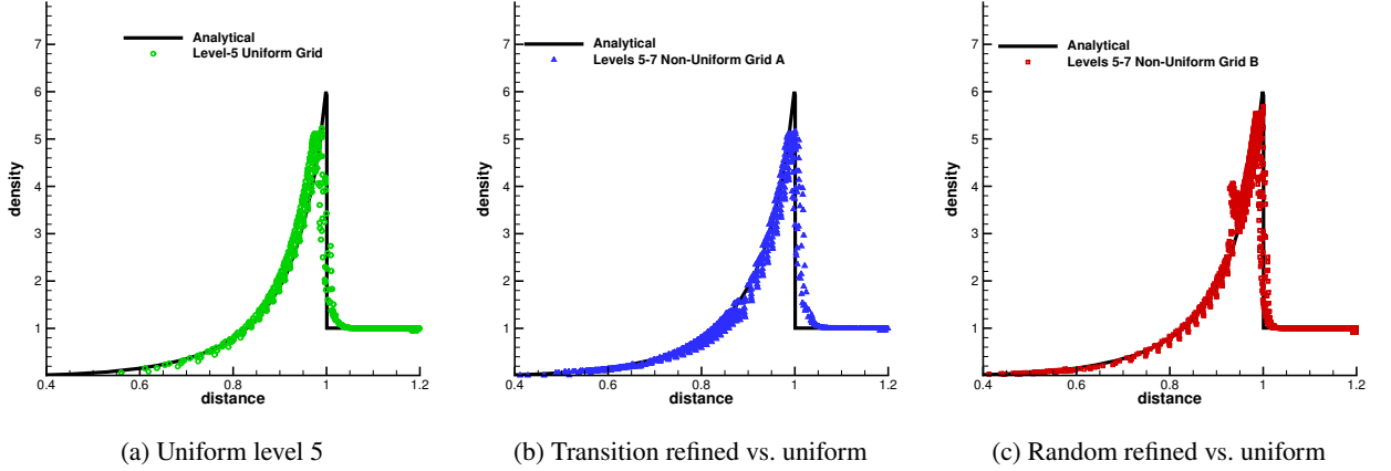
Figure 6: Radial density profiles at t = 1.0 for the Sedov blast wave problem. Results from the three configurations are compared against the exact analytical solution.
