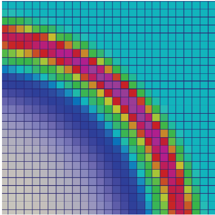
Eulerian
