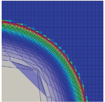
Lagrangian
