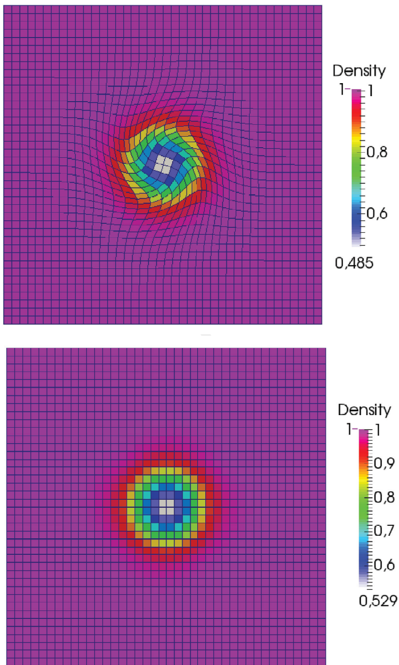
Figure 11: Density map, centered on the vortex eye, computed at time t = 1 for the 2D isotropic vortex test case: Lagrangian numerical solution (top) and Eulerian solution (bottom).
