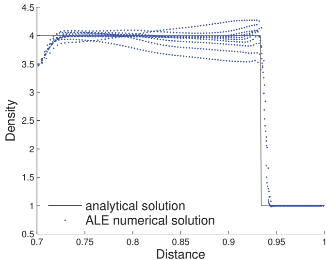
Figure 16: Density in all the cells as function of the cell center x-coordinate versus analytical solution at the computational time t = 0.7 - ALE Framework
