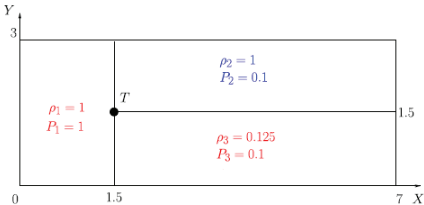
Figure 17: Initialization of the single material triple point problem
