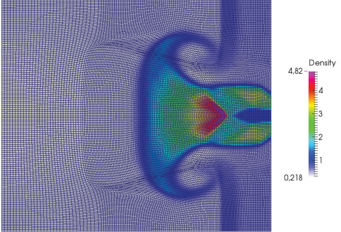
Figure 18: Density map and Mesh computed for the single material triple point test case at the computational time t_{\text{final}} = 5 . Standard ALE computation with \vec{w}_r = 0.3 \vec{v}_r
