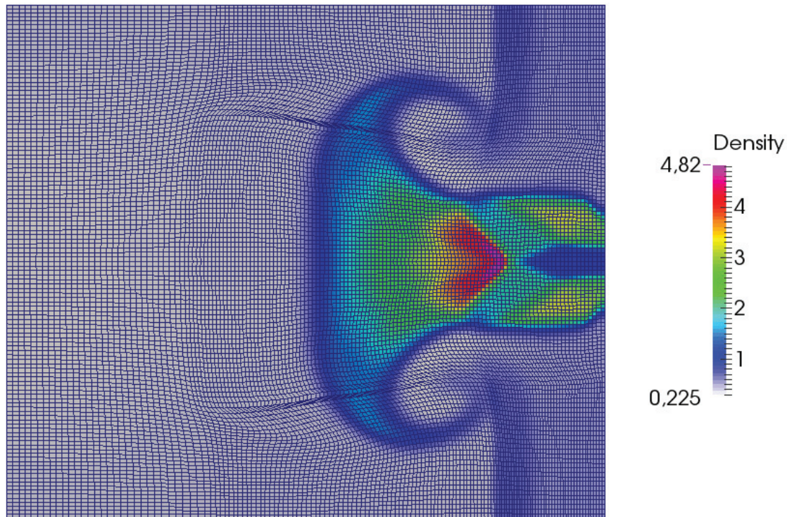
Figure 20: Density map and Mesh computed for the single material triple point test case at the computational time t_{\text{final}} = 5 . ALE computation with the L.E.L. method.
