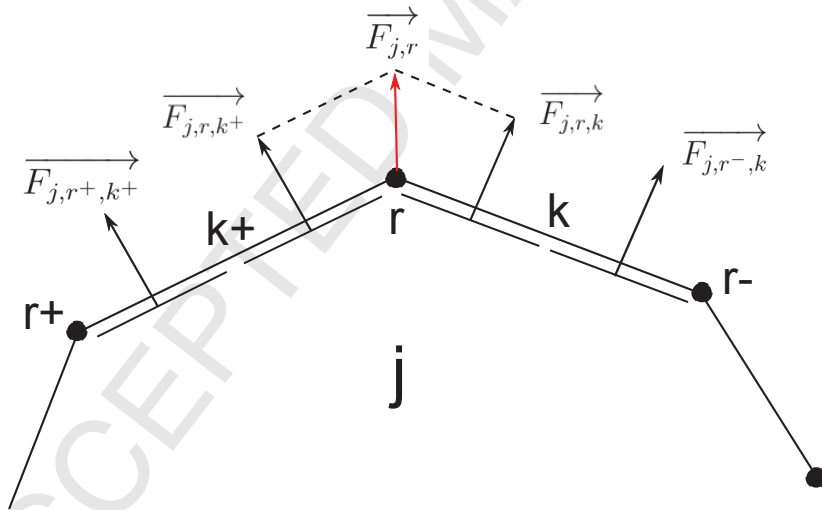
Figure 3: Representation of the nodal force on the node 'r', and of the edge forces applied on the edges connected to the node 'r'
