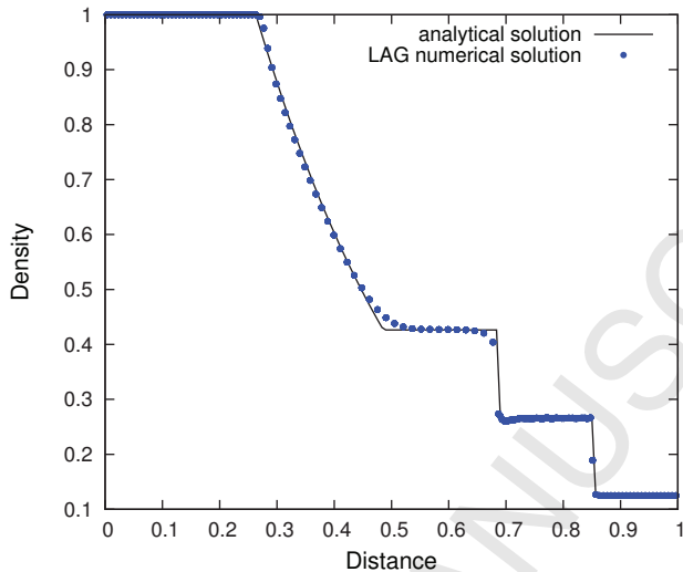
Figure 5: Comparison of the Lagrangian density profile computed at t_{\text{final}} = 0.2 with the analytical solution
