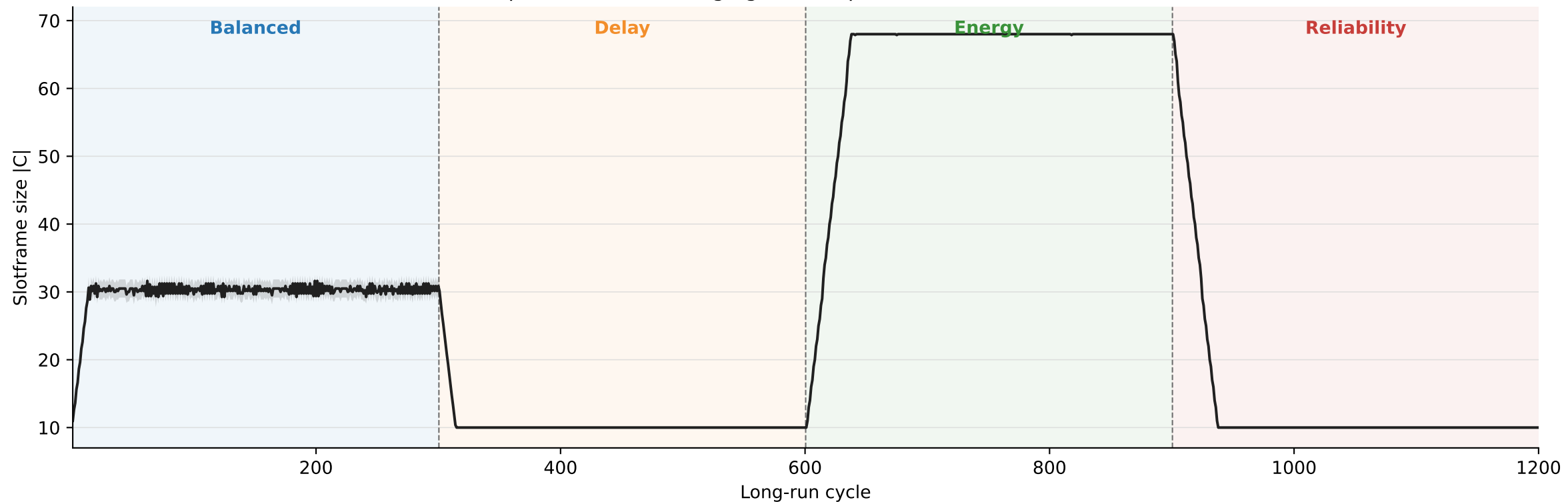
Slotframe adaptation under changing user requirements (8-seed mean and 95% CI)
