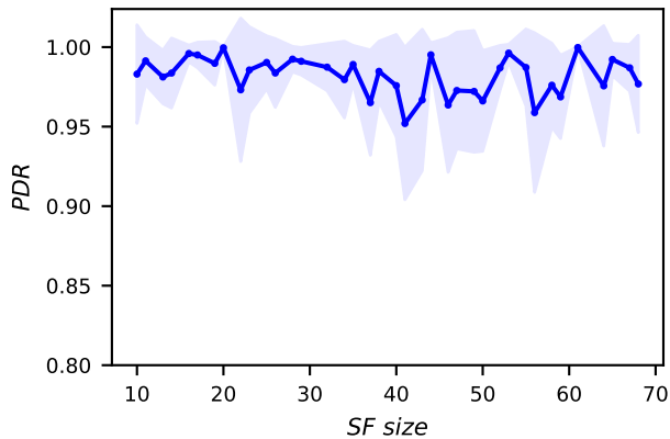
Network avg. PDR vs. SF size
