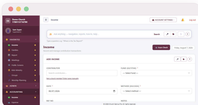
Income entry with contributor search, funds, and one-click “Scan Check” AI capture.
