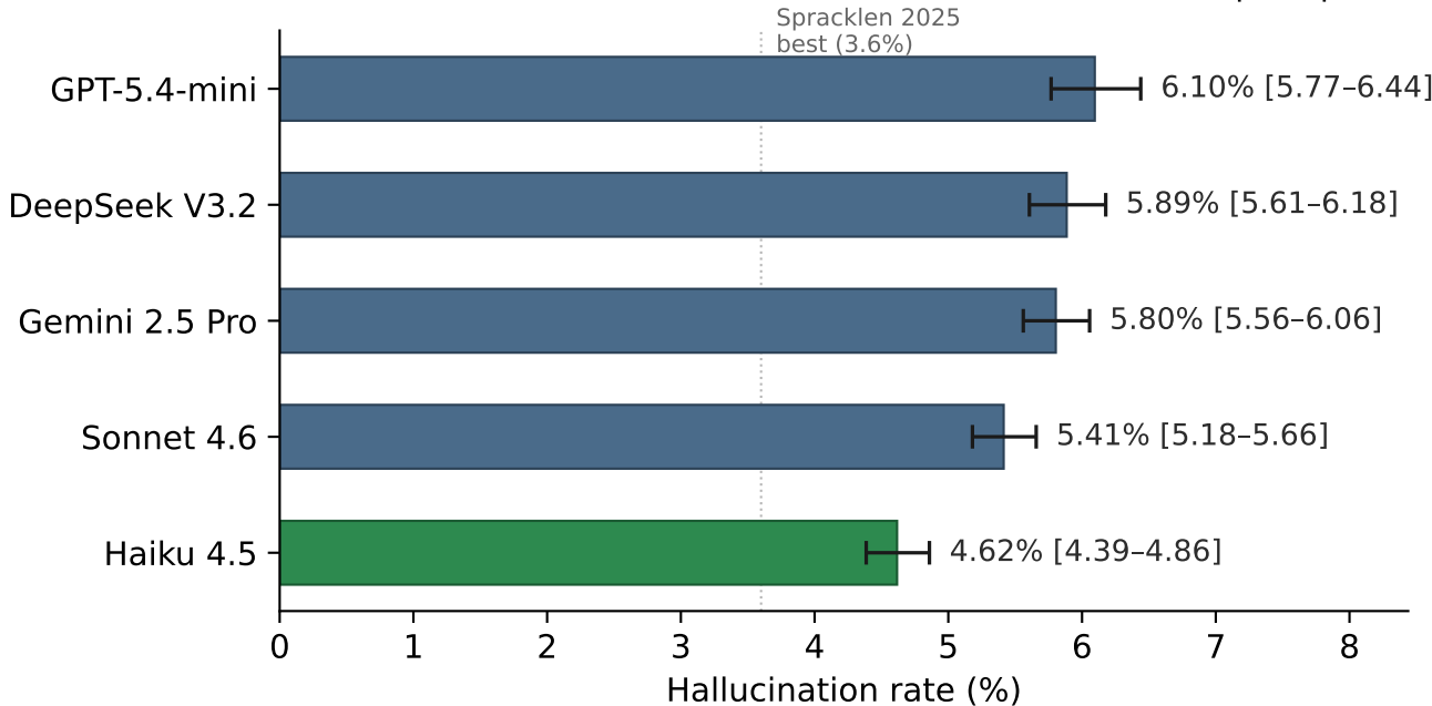
Hallucination rates across 5 frontier 2026 models (n≈40k prompts/model, 95% Wilson CIs)
