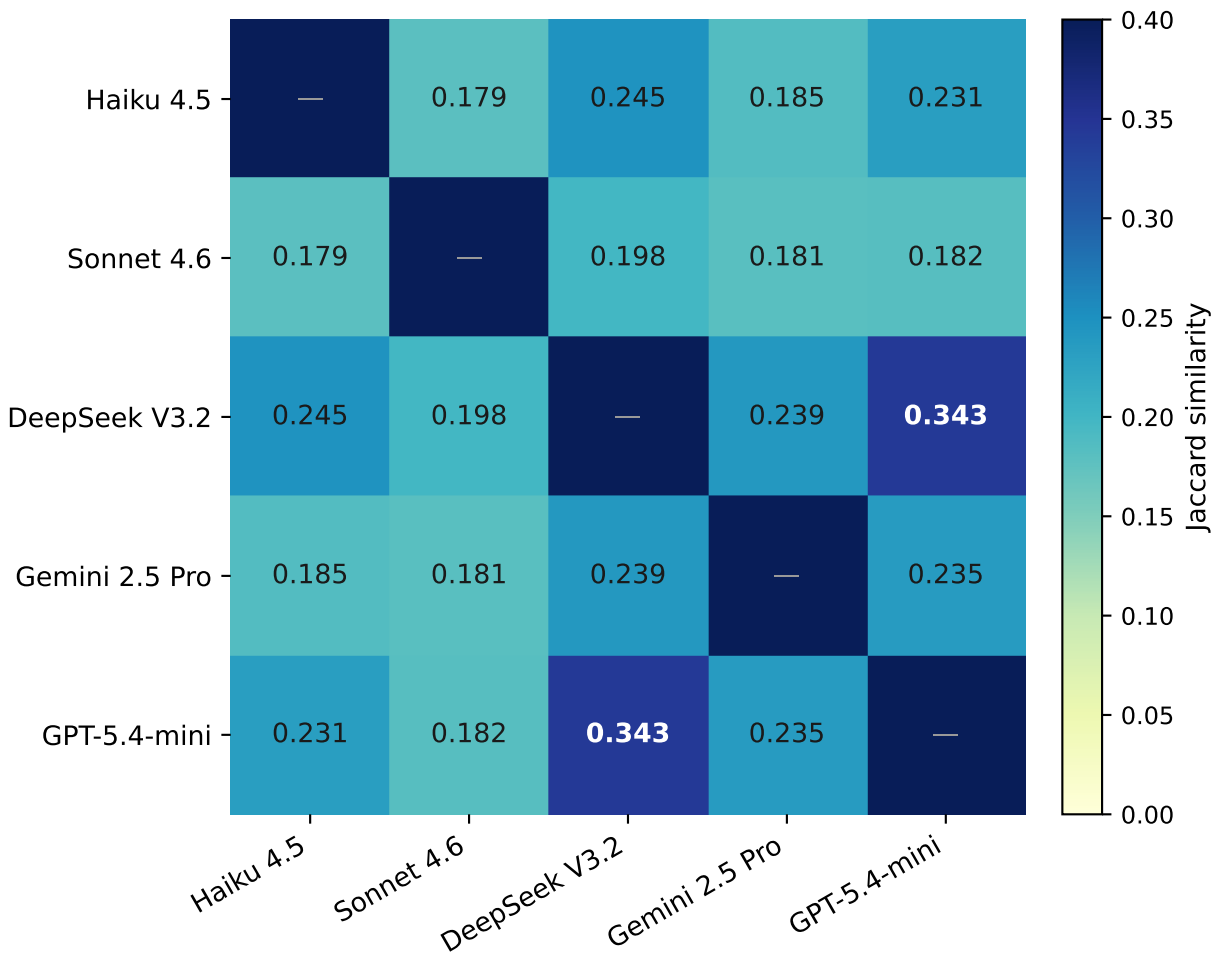
Pairwise Jaccard similarity of hallucinated package sets
