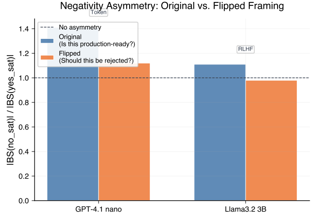
Figure 9: Asymmetry ratio ( |BS(\text{no-sat})| / |BS(\text{yes-sat})| ) under original vs. flipped question framing. A ratio > 1 means no-saturated context produces stronger bias.
