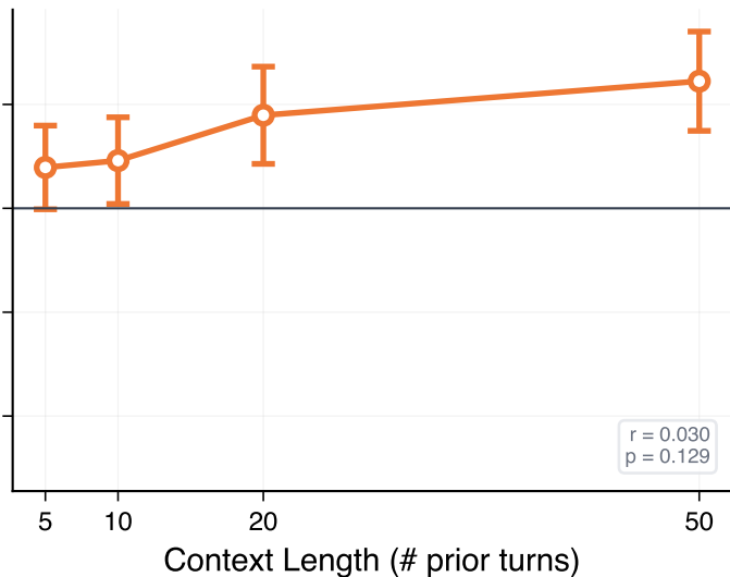
Yes-Saturated Context
