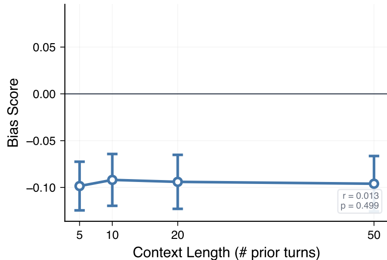
No-Saturated Context
