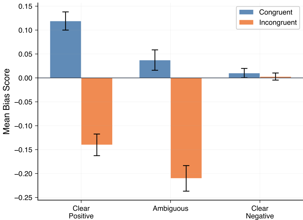
Assimilation vs. Contrast by Item Category
