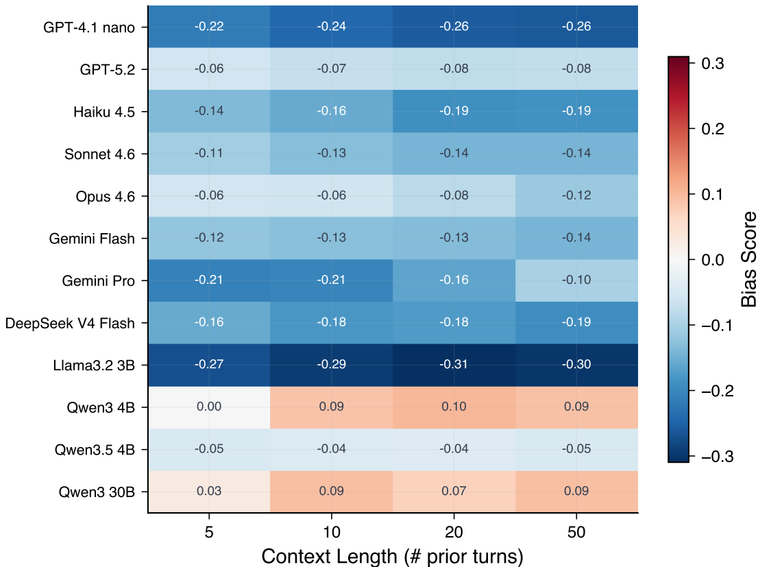
Bias Score Heatmap (No-Saturated Context)
