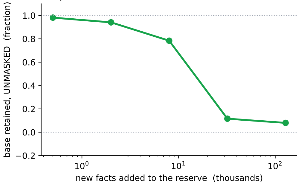
Always-on (soft): base retention falls with load (no mask/task-ID)
