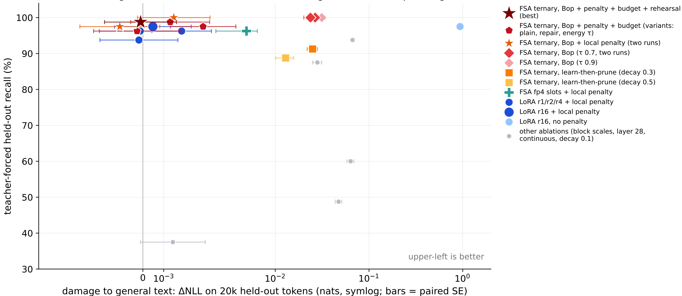
Recall vs damage on the real 8B model (40 facts, single seed; seeds pending)
