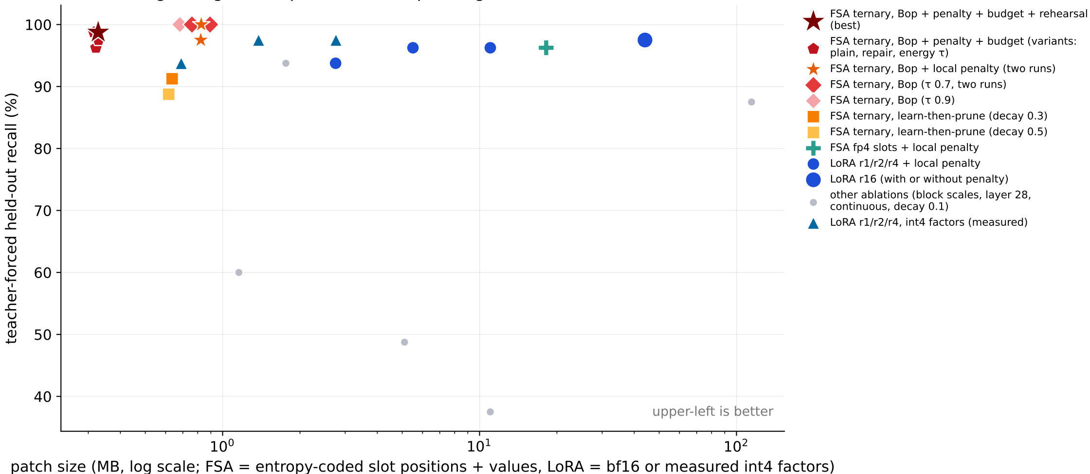
Patch storage (single seed per run; seeds pending)
