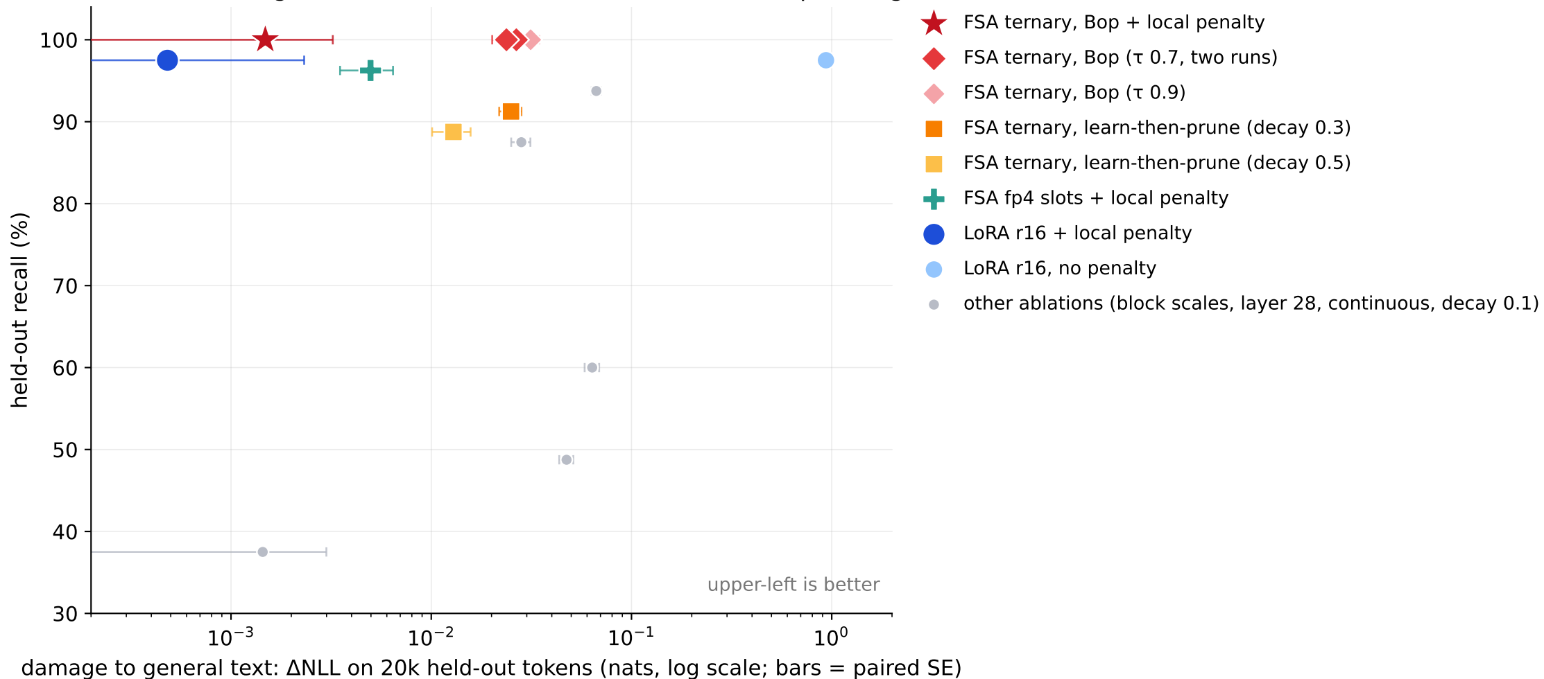
Recall vs damage on the real 8B model (40 facts, held-out phrasings)
