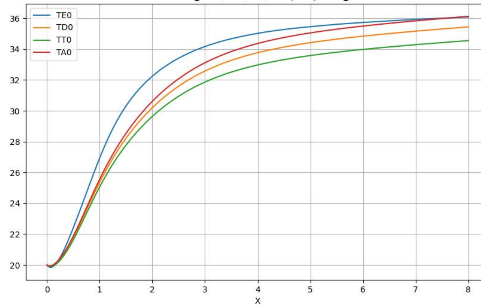
Title: @TE0,TD0,TT0,TA0 [keV] vs t@
