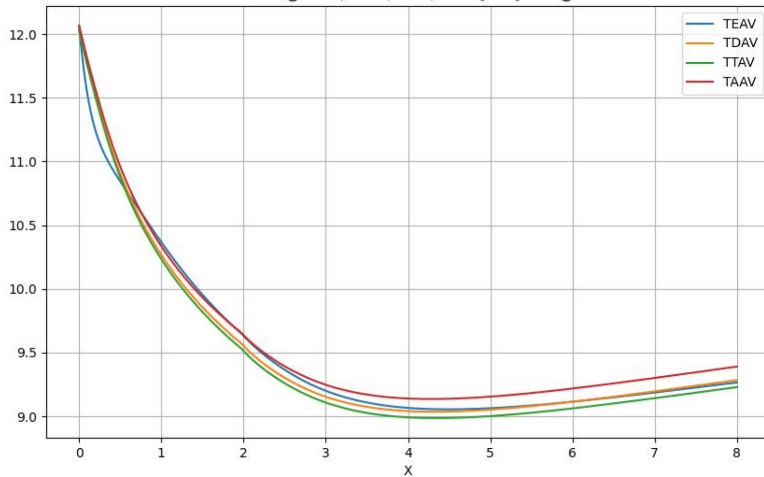
Title: @TEAV,TDAV,TTAV,TAAV [keV] vs t@
