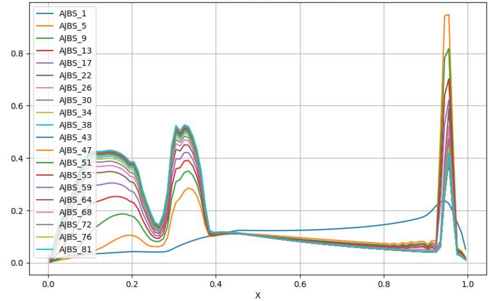
Title: @AJBS [MA/m 2 ] vs r@
