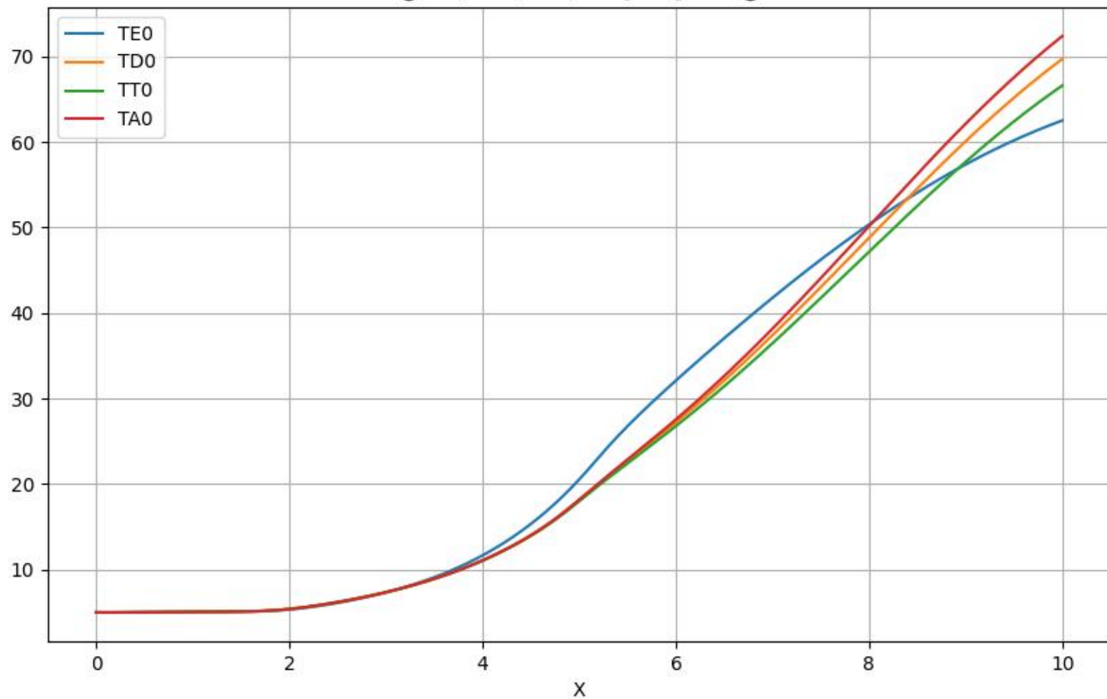
@TE0,TD0,TT0,TA0 [keV] vs t@
