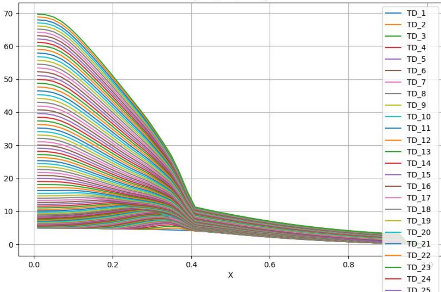
@TD [keV] vs r@
