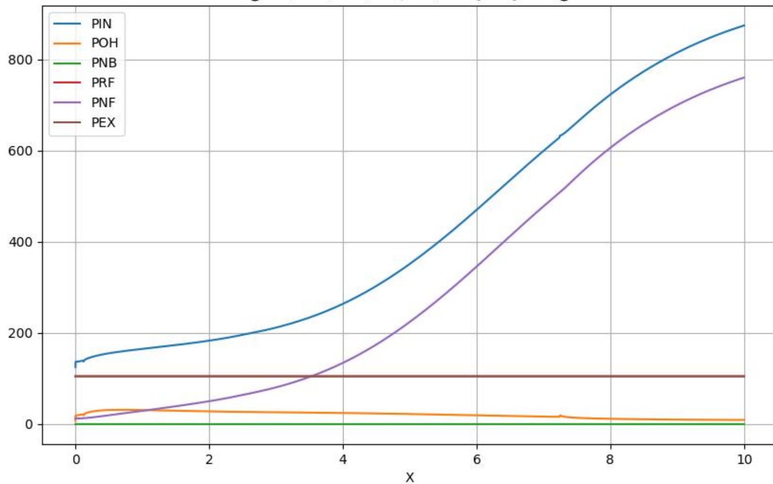
@PIN,POH,PNB,PRF,PNF,PEX [MW] vs t@
