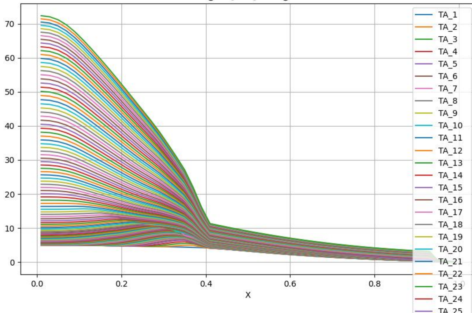
@TA [keV] vs r@
