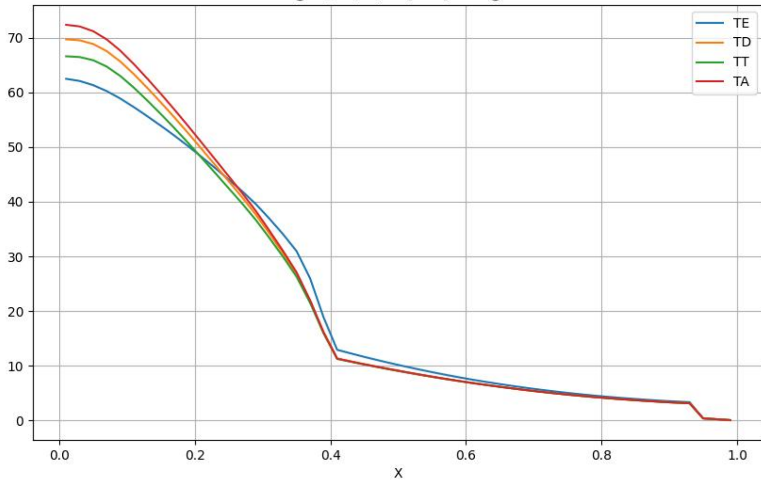
@TE,TD,TT,TA [keV] vs r@
