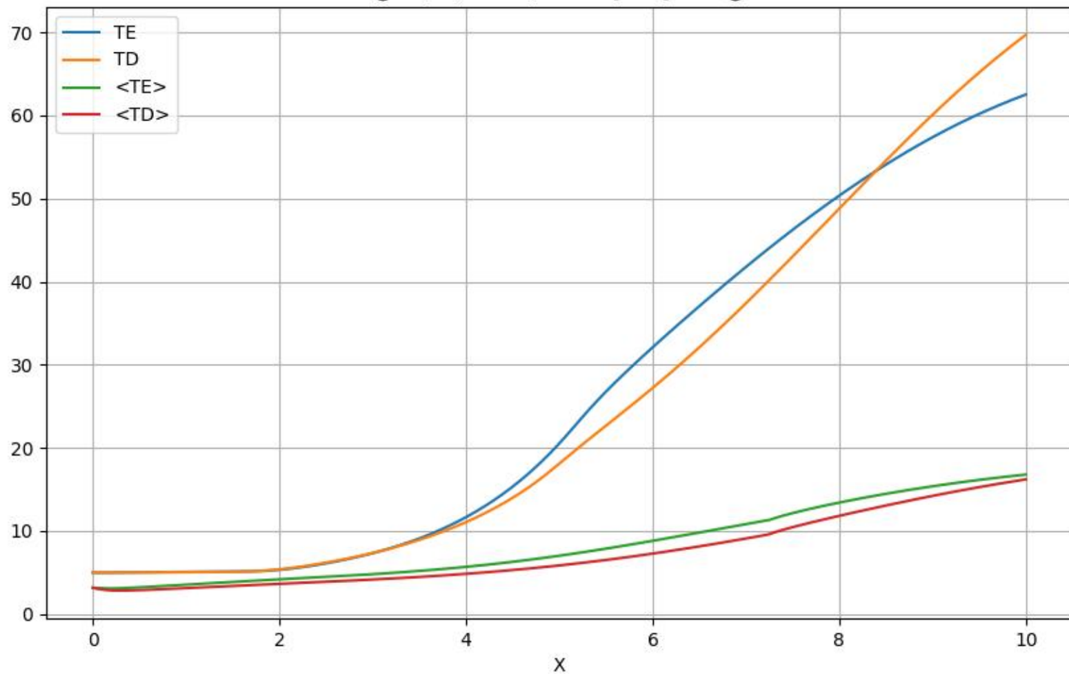
@TE,TD,<TE>,<TD> [keV] vs t@
