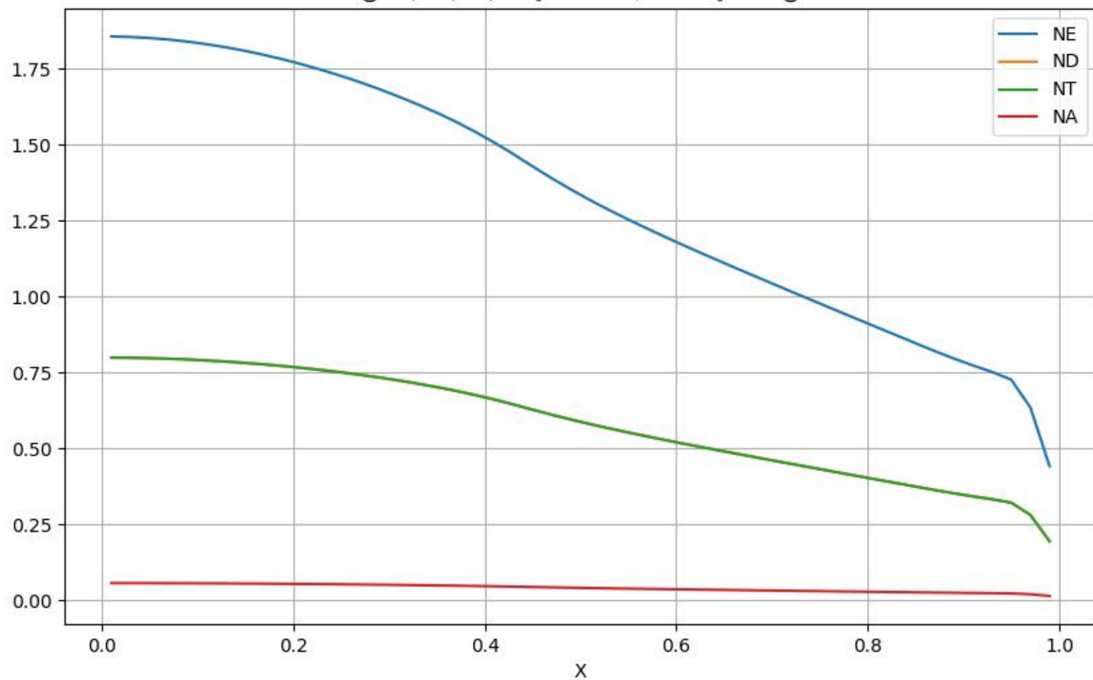
@NE,ND,NT,NA [10+20=/m+3=] vs r@
