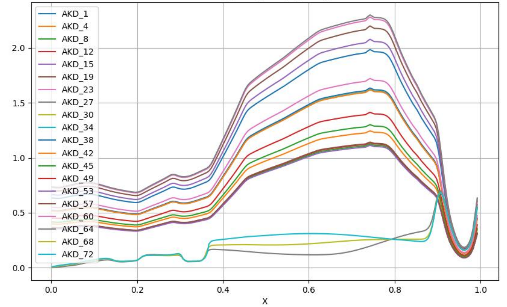
Title: @AKD [m^2/s] vs r@
