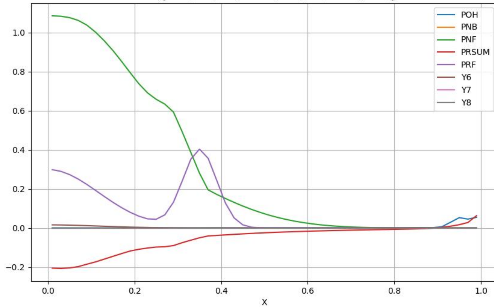
Title: @POH,PNB,PNF,PRSUM,PRF [MW/m+3=] vs r@
