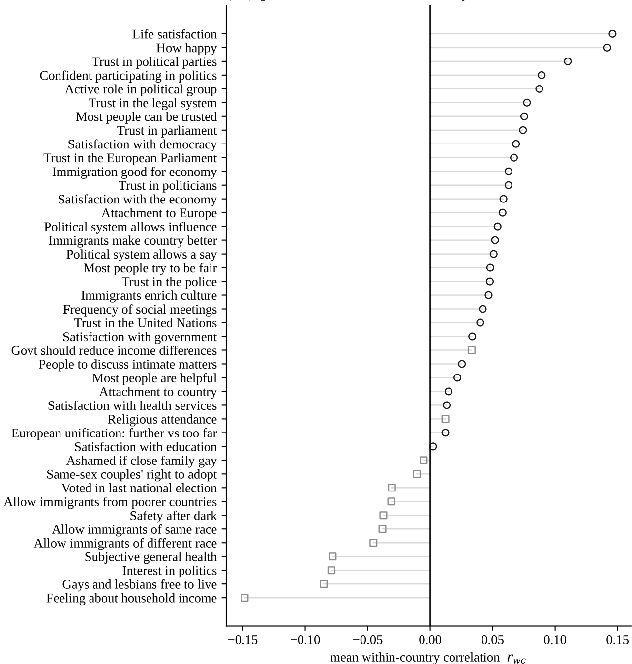
(A3) per-item individual-level recovery, Qwen 1P
