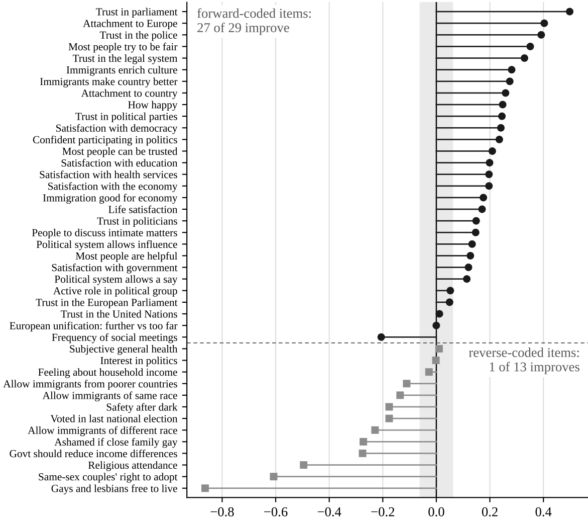
country-label effect per item ( r_{bc} , Fisher z ): with the label minus without (b) added to sparse base (c) removed from full profile
