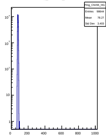
Ping_Chn55_HG
