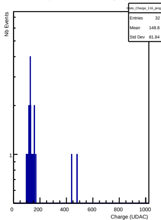
Charges in channel 116 (ping)
