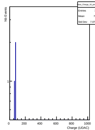
Charges in channel 18 (ping)
