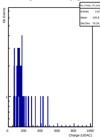
Charges in channel 125 (ping)
