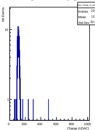
Charges in channel 14 (ping)
