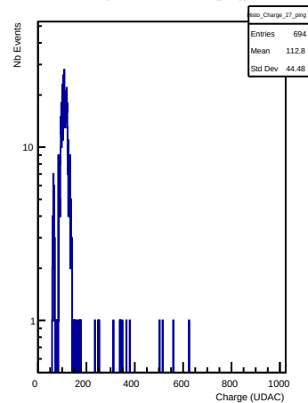
Charges in channel 27 (ping)
