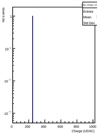
Charges in channel 137 (ping)
