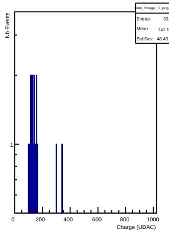
Charges in channel 57 (ping)
