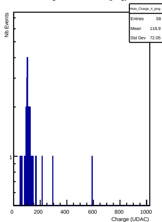
Charges in channel 4 (ping)
