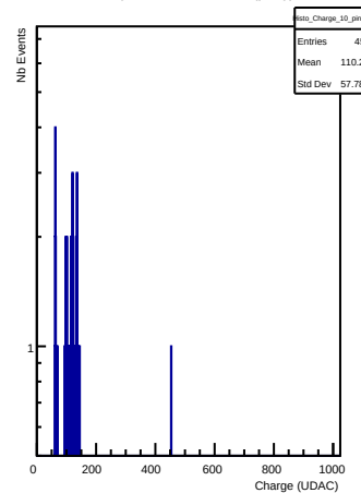
Charges in channel 10 (ping)
