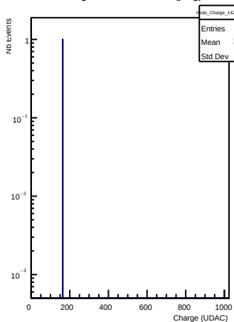
Charges in channel 142 (ping)
