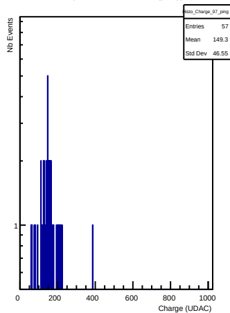
Charges in channel 97 (ping)
