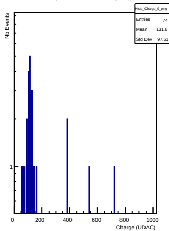
Charges in channel 0 (ping)
