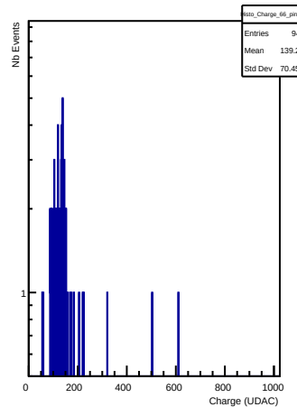
Charges in channel 66 (ping)
