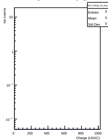
Charges in channel 94 (ping)
