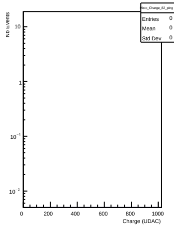
Charges in channel 82 (ping)
