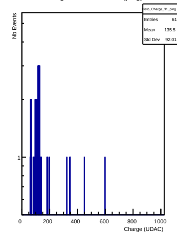
Charges in channel 31 (ping)
