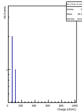
Charges in channel 26 (ping)
