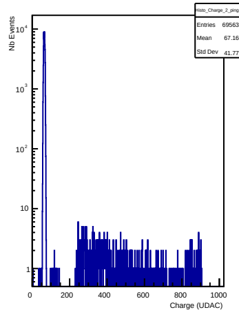
Charges in channel 2 (ping)
