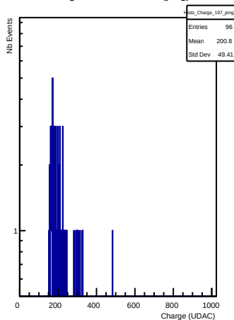
Charges in channel 197 (ping)
