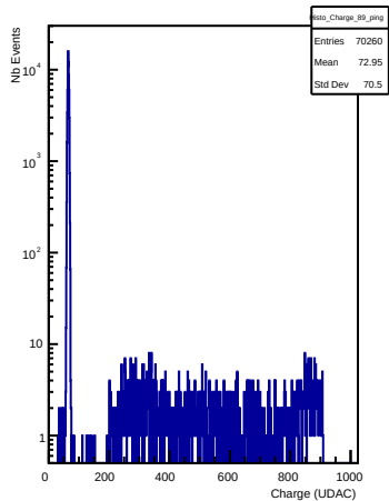
Charges in channel 89 (ping)
