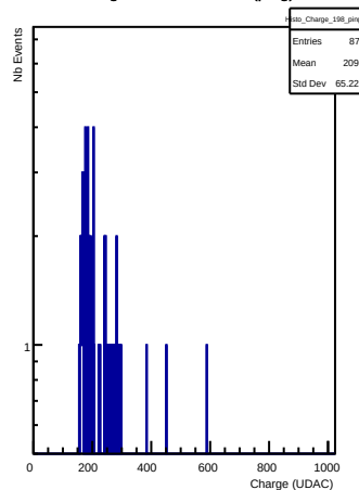
Charges in channel 198 (ping)
