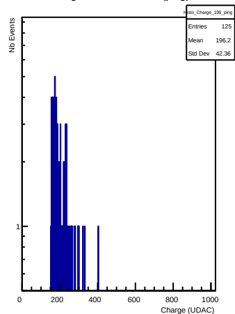
Charges in channel 199 (ping)
