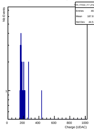
Charges in channel 217 (ping)
