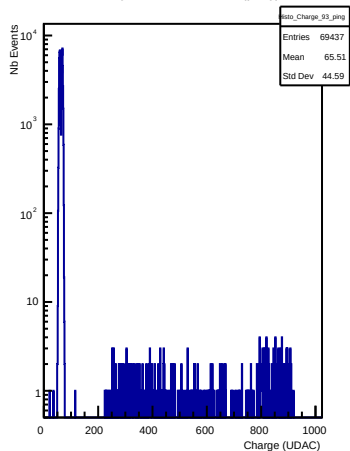
Charges in channel 93 (ping)
