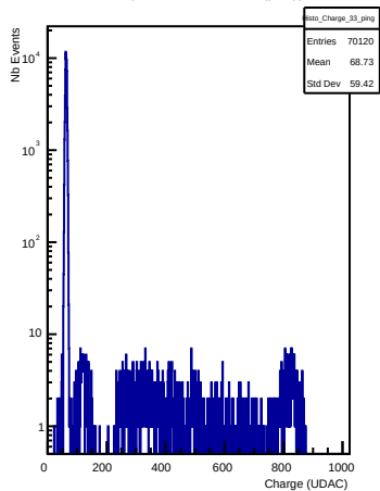
Charges in channel 33 (ping)
