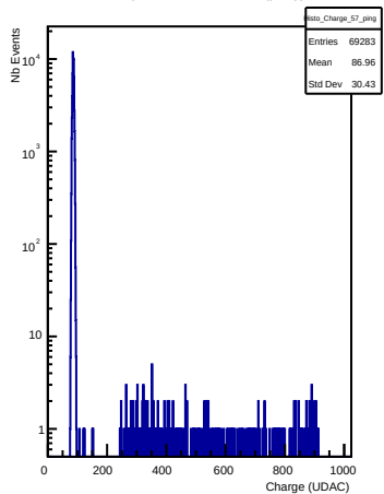
Charges in channel 57 (ping)
