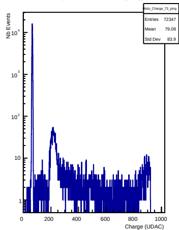
Charges in channel 73 (ping)
