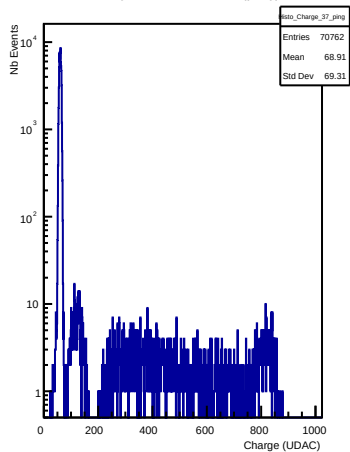
Charges in channel 37 (ping)
