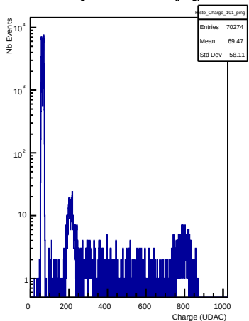
Charges in channel 101 (ping)
