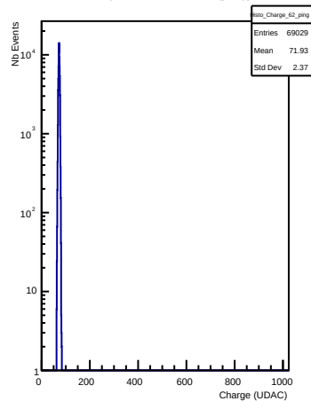
Charges in channel 62 (ping)
