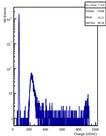
Charges in channel 77 (ping)
