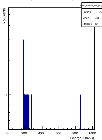
Charges in channel 145 (ping)
