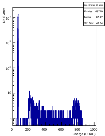
Charges in channel 97 (ping)
