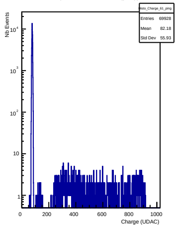
Charges in channel 61 (ping)
