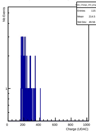
Charges in channel 253 (ping)
