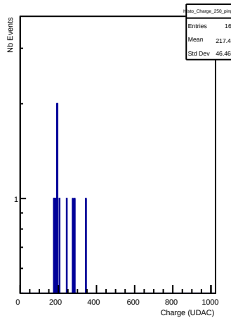
Charges in channel 250 (ping)
