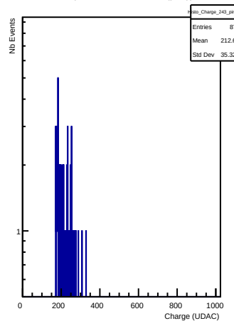
Charges in channel 243 (ping)
