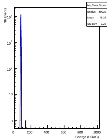
Charges in channel 58 (ping)
