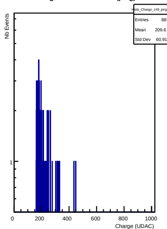
Charges in channel 149 (ping)
