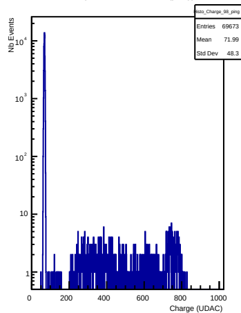
Charges in channel 98 (ping)
