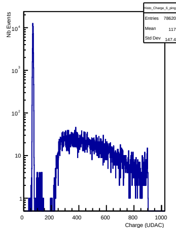
Charges in channel 6 (ping)
